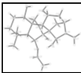
Fig. 1. A view of the molecular structure of compound. Displacement ellipsoids are drawn at the 50% probability level.
