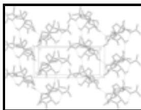
Fig. 2. The crystal packing of compound, viewed along the a axis, showing the O—H...O hydrogen bonds as dashed lines.
